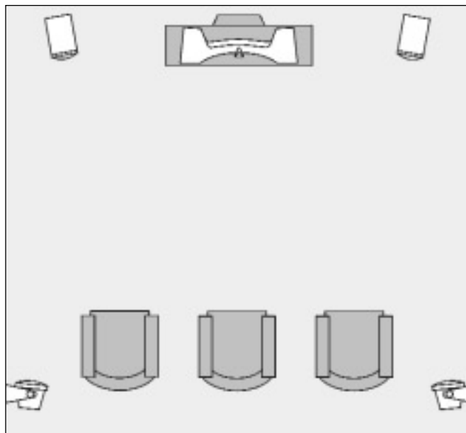
Figure 13. Scenario speakers as front channels, MartinLogan Cinema as the center channel, MartinLogan Scripts as side surround (effects) channels.
